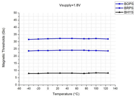
Magnetic threshold value vs temperature @ V_{DD}=1.8\text{V}
