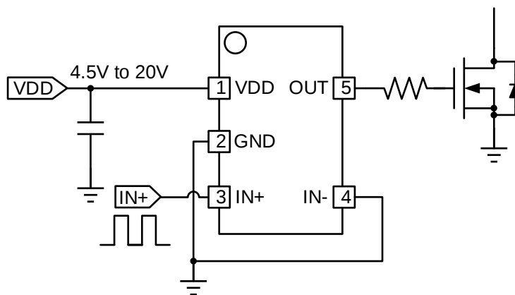
Using Non-Inverting Input
