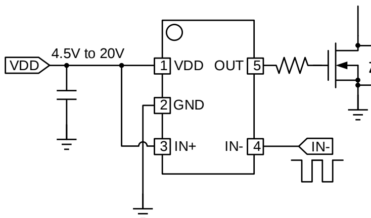
Using Inverting Input
