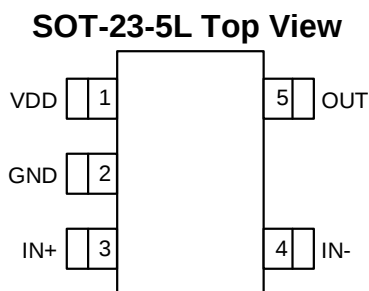
Pin Functions
