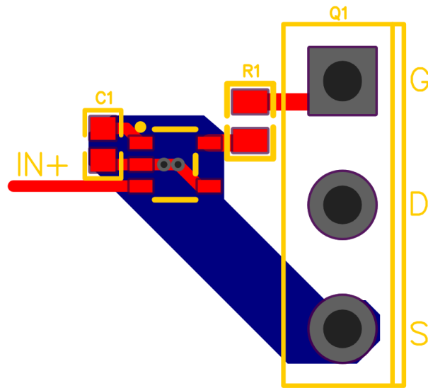
Layout Example for SL27517A
